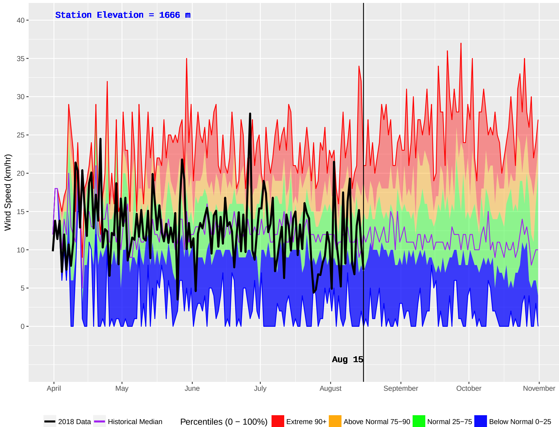
BALDFACE (221) : Historical (1992–2016) and Current (2018) Daily Wind Speed
