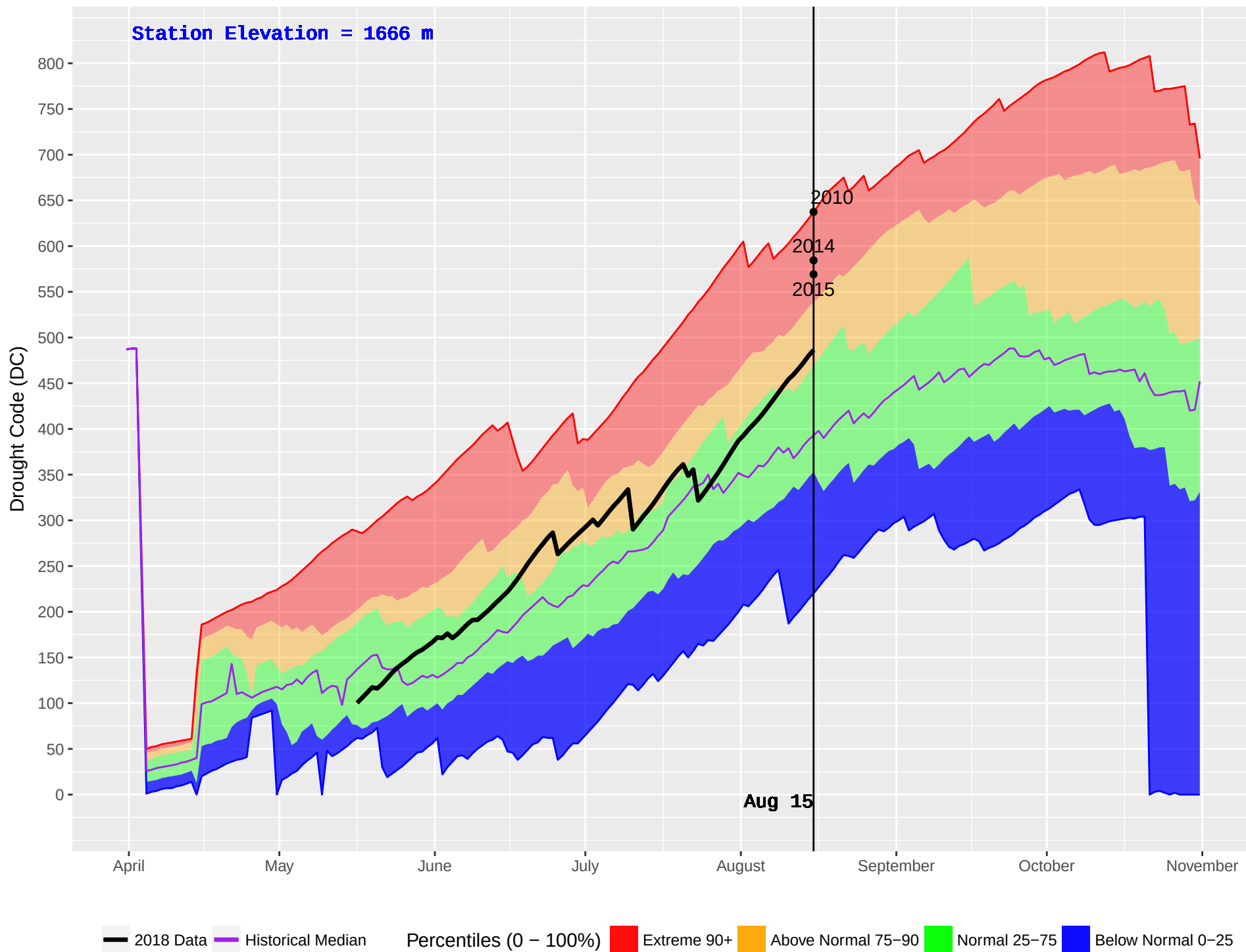
BALDFACE (221) : Historical (1992–2016) and Current (2018) Daily Drought Code (DC)
