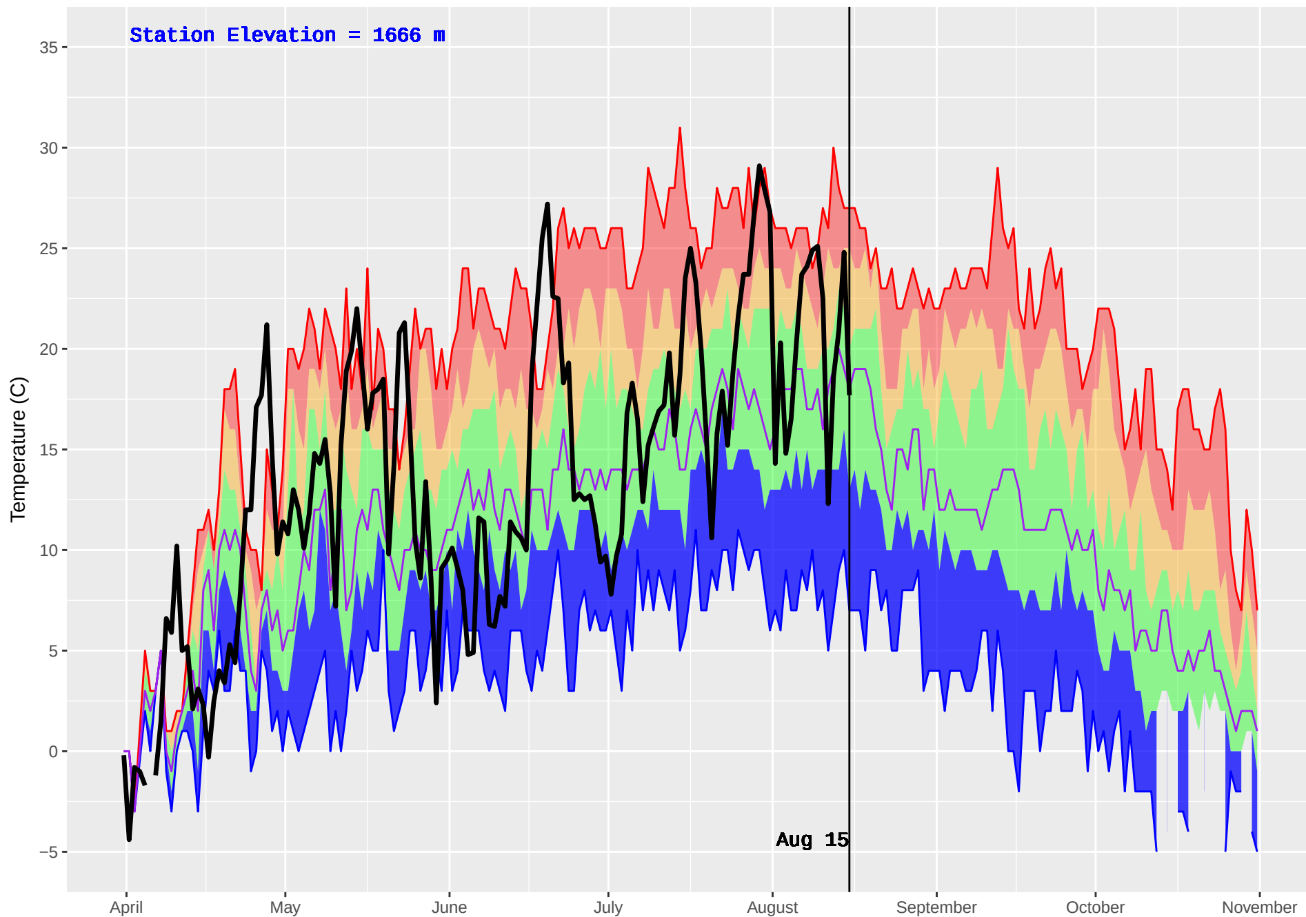
BALDFACE (221) : Historical (1992–2016) and Current (2018) Daily Temperature
