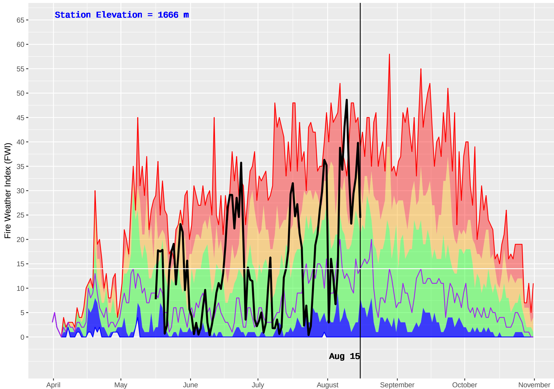
BALDFACE (221) : Historical (1992–2016) and Current (2018) Daily Fire Weather Index (FWI)
