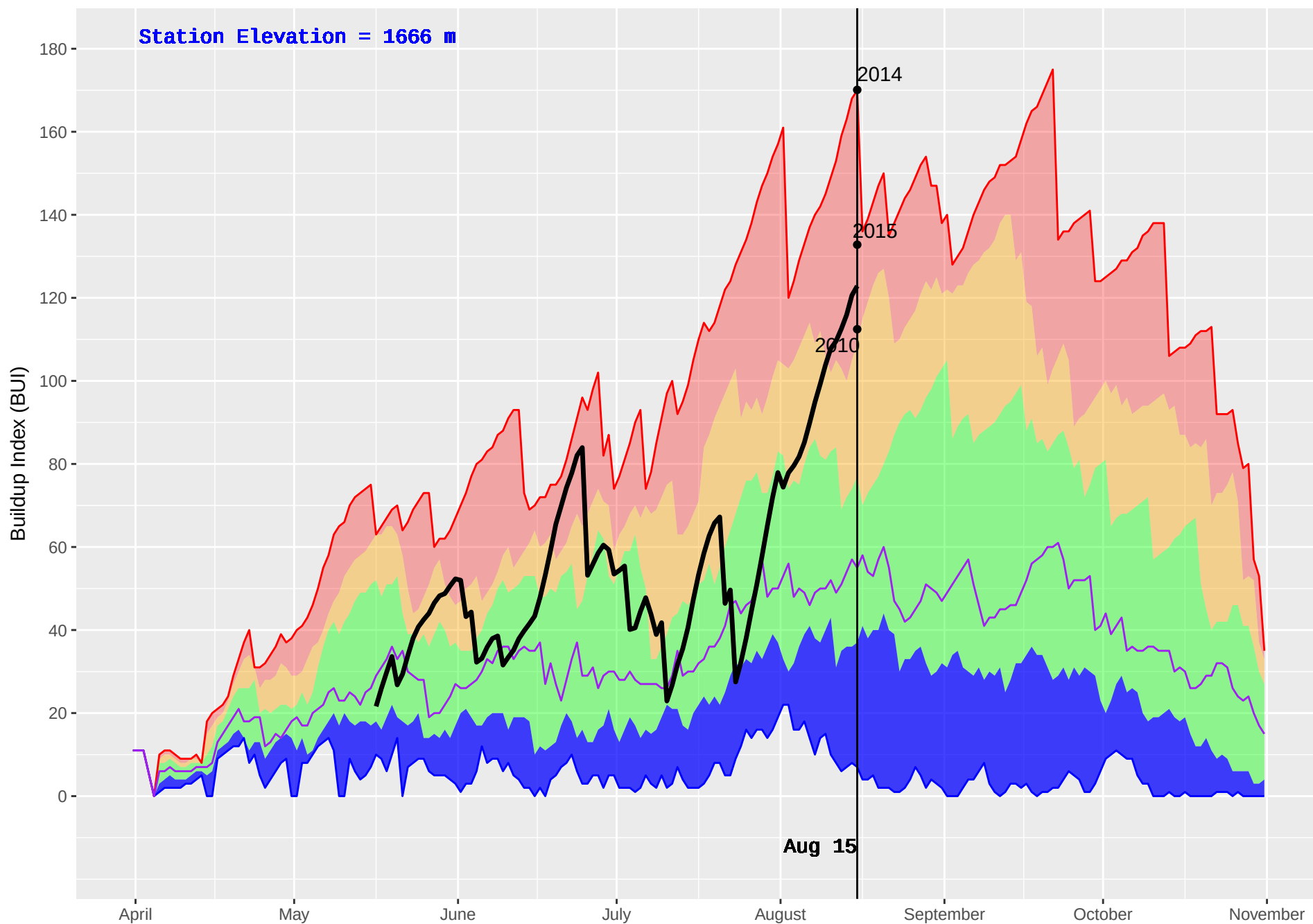
BALDFACE (221) : Historical (1992–2016) and Current (2018) Daily Buildup Index (BUI)
