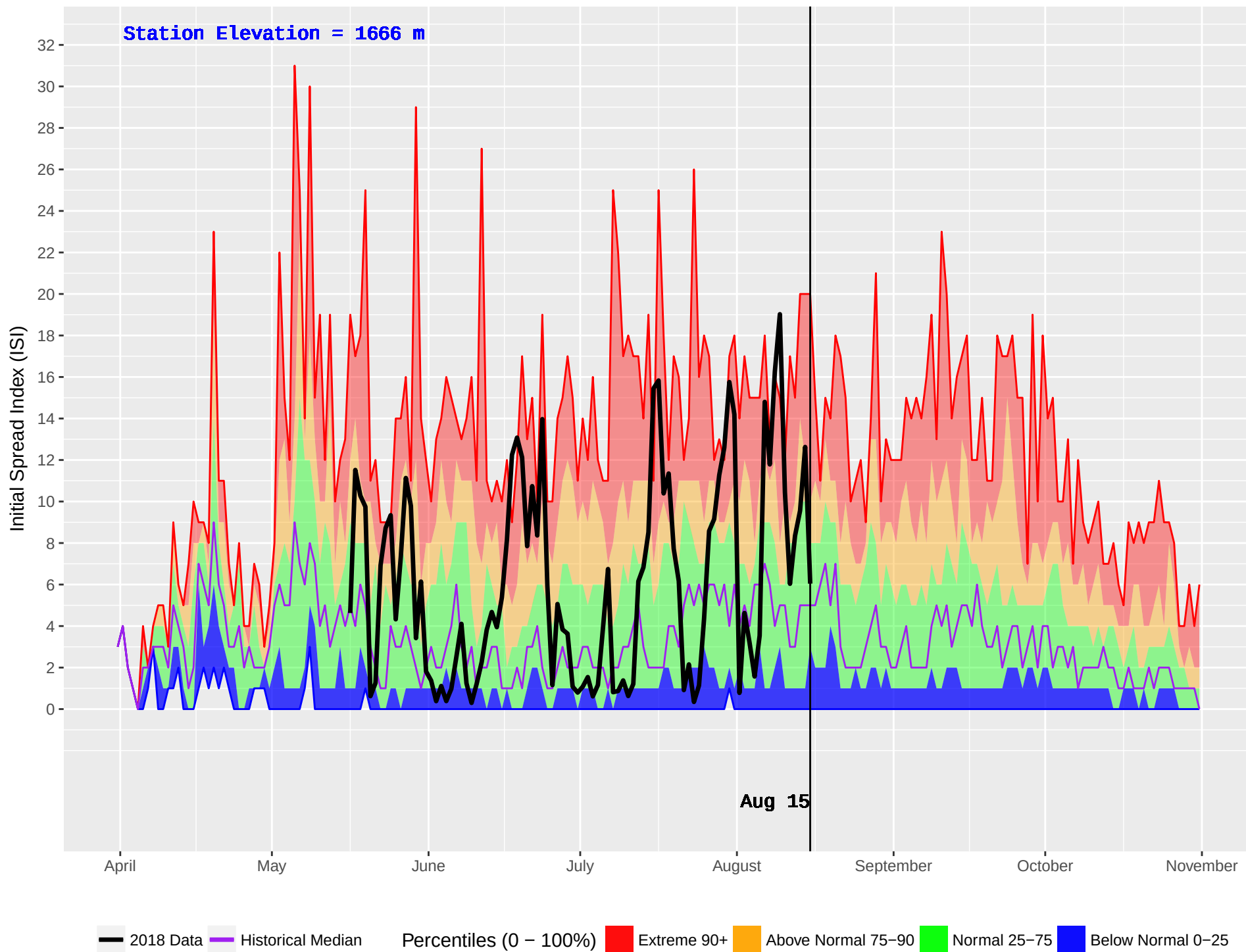
BALDFACE (221) : Historical (1992–2016) and Current (2018) Daily Initial Spread Index (ISI)
