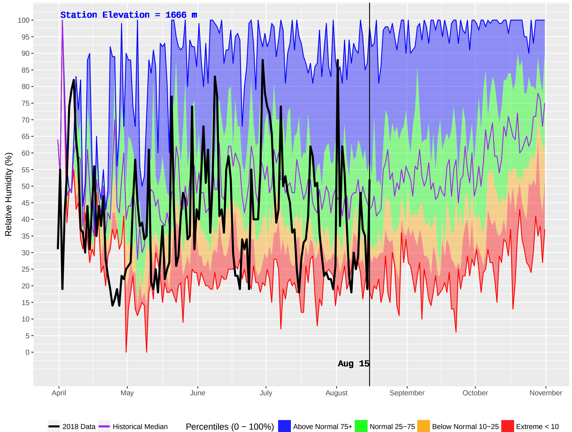
BALDFACE (221) : Historical (1992–2016) and Current (2018) Daily Relative Humidity
